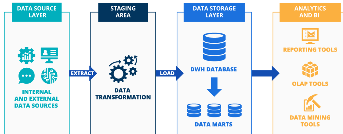
A SAMPLE DATA WAREHOUSE SOLUTION ARCHITECTURE
